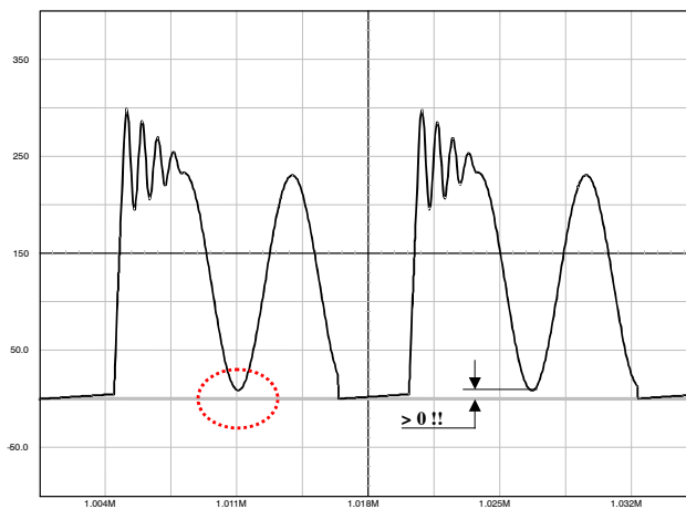
Figure 46. The Drain-source Wave Shall always be Positive
